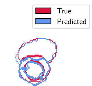
segmentations
